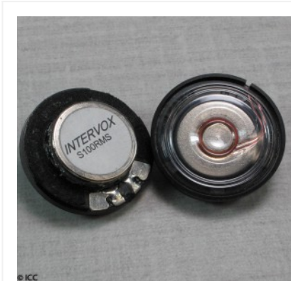
SUB-MINIATURE LOW PROFILE ROUND SPEAKER
