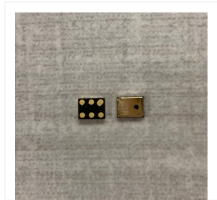
MEMS TOP PORT DIGITAL MICROPHONE
